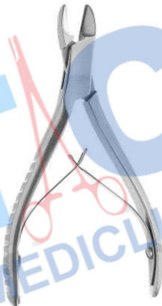
Delicate Wire Cutter TC10-1209 12.5cm Side cutting w/ carbide inserts max capacity. 0.7mm 028"
