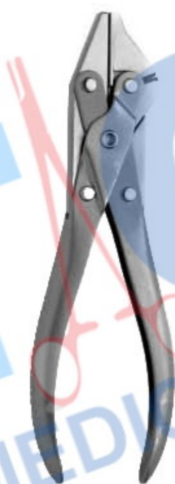
Flat Nose Plier TC10-1036 18.5cm parallel grip, incorporated cutter, for hard wires up to 1.6mm
